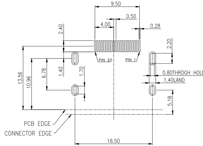
RECOMMENDED P.C.B. LAYOUT TOP VIEW, THK=1.6MM, TOL:±0.05mm
